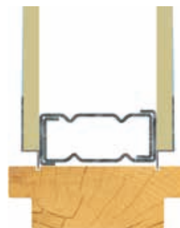
DETAIL AT DOOR JAMB
