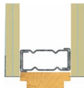
P28: DETAIL AT DOOR JAMB
