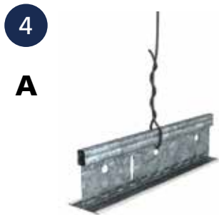
4 A Rondo 120 soft galvanised wire secured with three tight 360° turns
